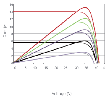
Current-Voltage & Power-Voltage Curves (470W)
